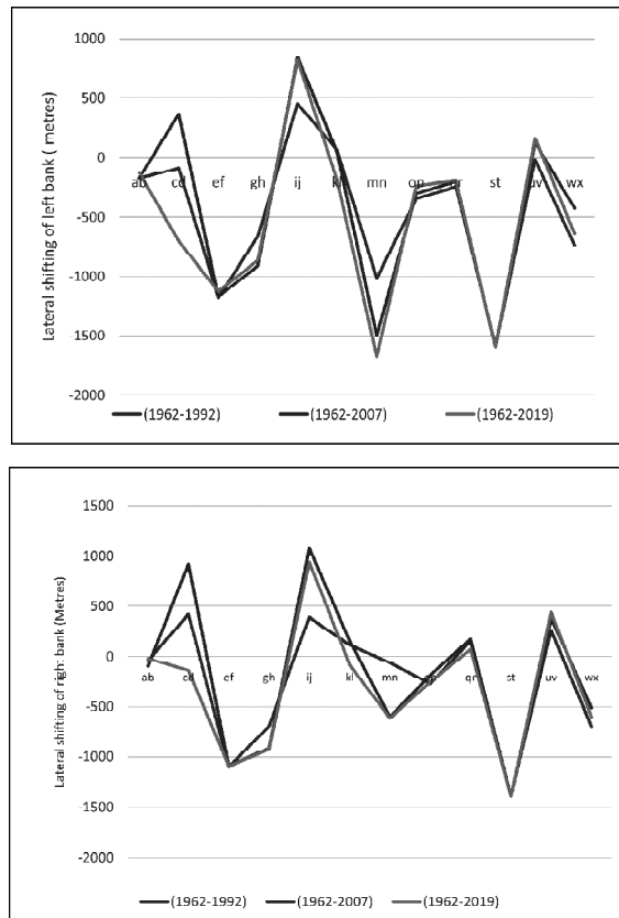
Fig.4. Lateral shift of left and right bank of the Kaljani river
